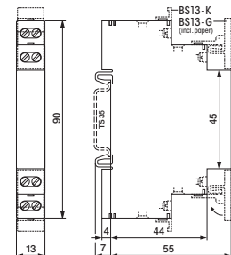
fig. 3. Dimension (mm)
