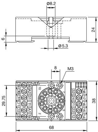
fig. 2. Dimensions (mm)
