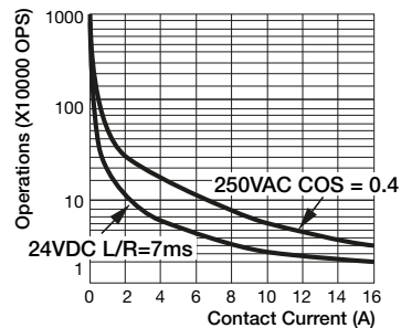
fig. 3. DC load limit curve
