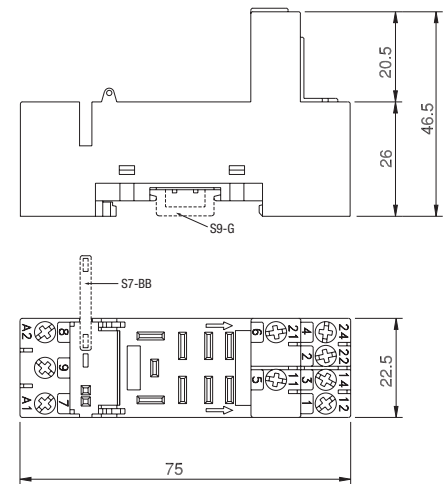
fig. 2. Dimensions (mm)
