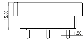
fig. 2. Dimensions (mm)
