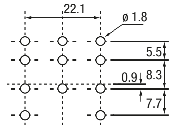
fig. 2. Dimensions (mm)
