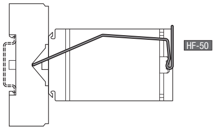
fig. 1. Mounting
