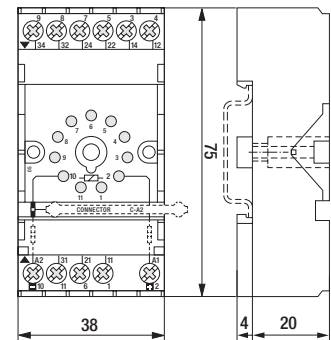
fig. 2. Dimensions (mm)
