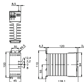
fig. 2. Dimensions (mm)
