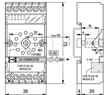
fig. 2. Dimensions (mm)
