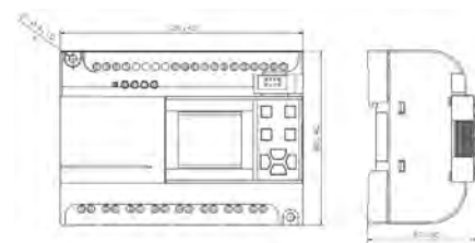
fig. 2. Dimension (mm)
