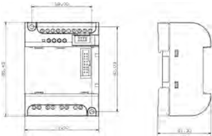
fig. 2. Dimension (mm)
