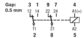
fig. 2. AC voltage endurance
