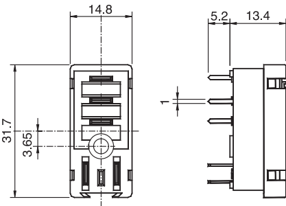
fig. 2. Dimensions (mm)
