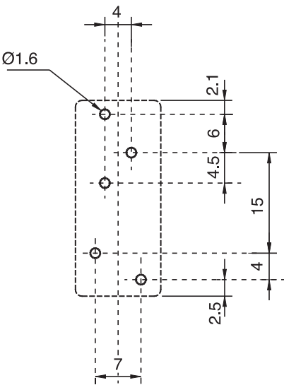
fig. 2. Dimensions (mm)
