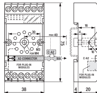
fig. 2. Dimensions (mm)
