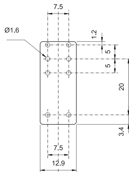
fig. 2. Dimensions (mm)
