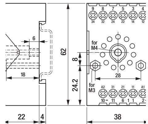
fig. 2. Dimensions (mm)
