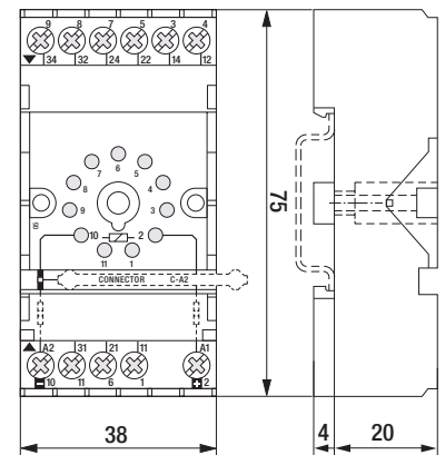
fig. 2. Dimensions (mm)
