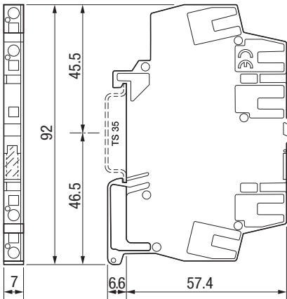
fig. 2. Dimensions (mm)
