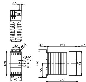
fig. 2. Dimensions (mm)
