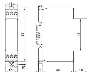
fig. 2. Dimensions (mm)
