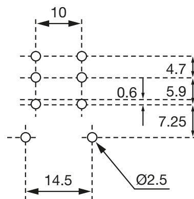
fig. 2. Dimensions (mm)
