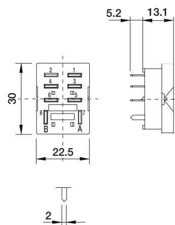
fig. 2. Dimensions (mm)
