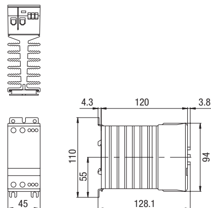
fig. 2. Dimensions (mm)
