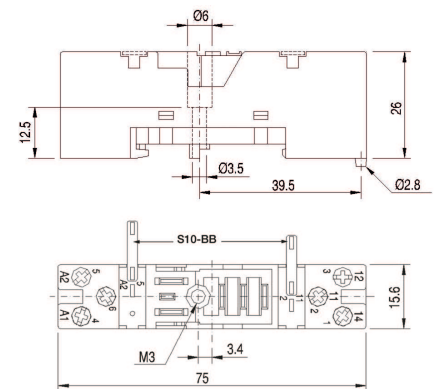
fig. 2. Dimensions (mm)
