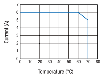
fig. 2. DC derating curve
