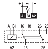
fig. 2. AC voltage endurance
