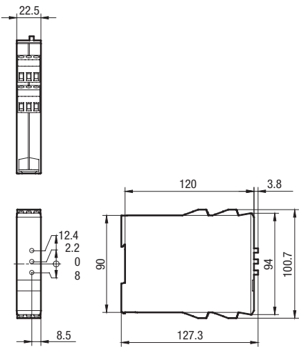
fig. 2. Dimensions (mm)
