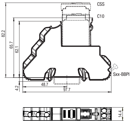
fig. 2. Dimensions (mm)
