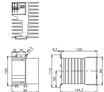
fig. 2. Dimensions (mm)
