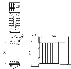
fig. 2. Dimensions (mm)
