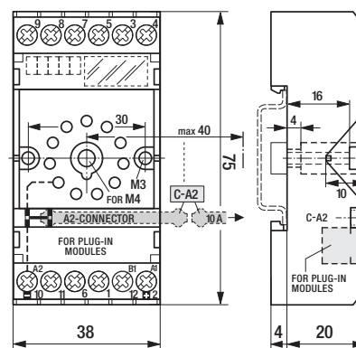
fig. 2. Dimensions (mm)
