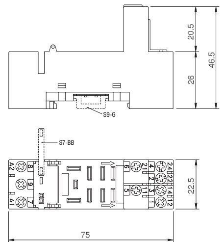
fig. 2. Dimensions (mm)
