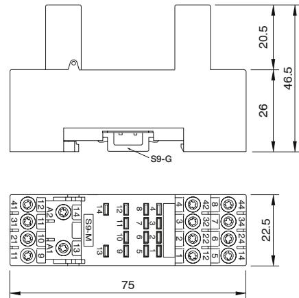
fig. 2. Dimensions (mm)
