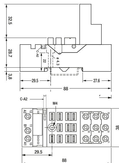
fig. 2. Dimensions (mm)
