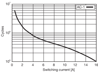
fig. 2. AC voltage endurance
