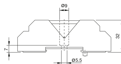
fig. 2. Dimensions (mm)
