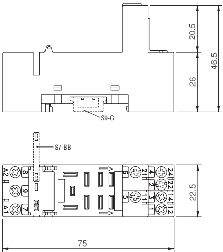
fig. 2. Dimensions (mm)
