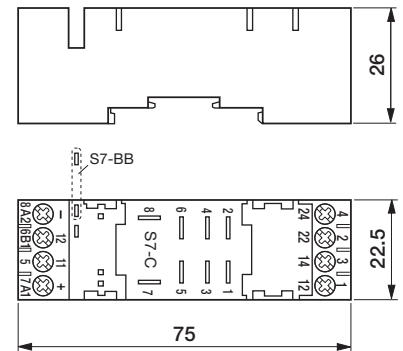
fig. 2. Dimensions (mm)
