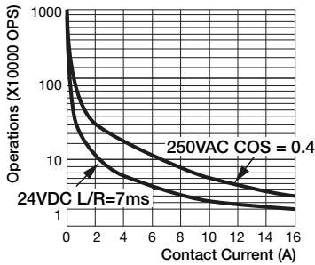
fig. 3. DC load limit curve
