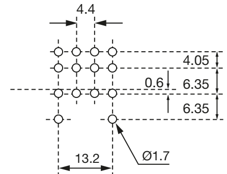
fig. 2. Dimensions (mm)
