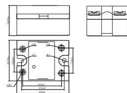
fig. 5. Dimension (mm)
