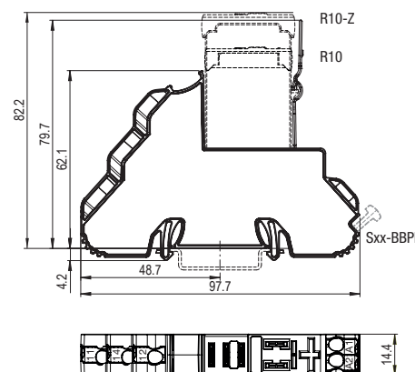
fig. 2. Dimension (mm)
