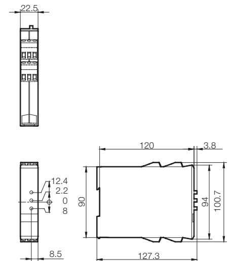
fig. 2. Dimension (mm)
