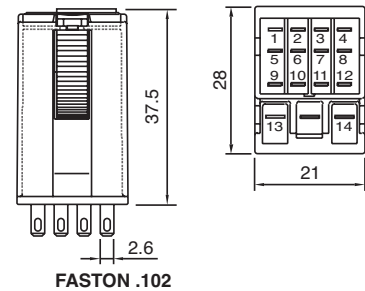
fig. 4. Dimension (mm)
