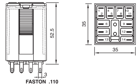
fig. 4. Dimension (mm)
