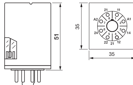
fig. 4. Dimension (mm)
