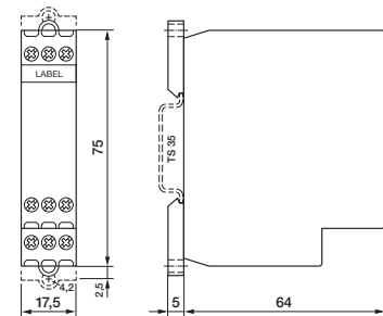
fig. 3. Dimension (mm)
