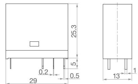
fig. 3. Dimension (mm)
