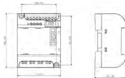
fig. 2. Dimensions (mm)
