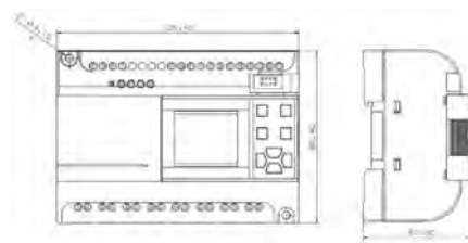
fig. 2. Dimensions (mm)
