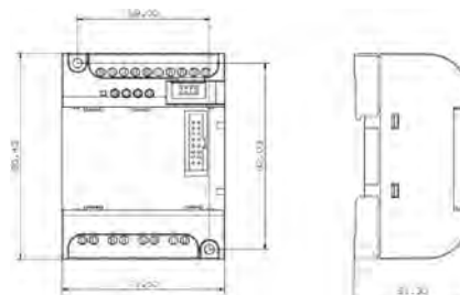
fig. 2. Dimensions (mm)
