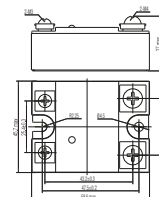
fig. 5. Dimension (mm)
