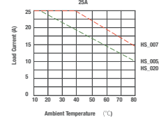
fig. 3. Thermal derating curve 40 A
