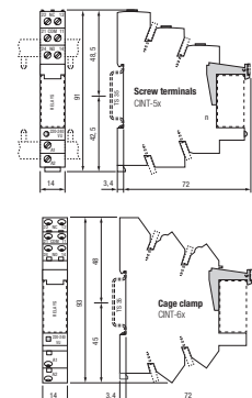
fig. 4. Dimension (mm)
