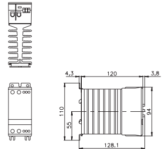
fig. 2. Dimension (mm)
