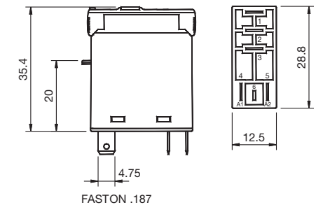
fig. 4. Dimension (mm)
