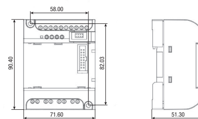
fig. 2. Dimension (mm)
