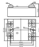
fig. 5. Dimension (mm)
